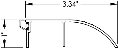
30 OUTSWING THRESHOLD Pemko 2051-T
