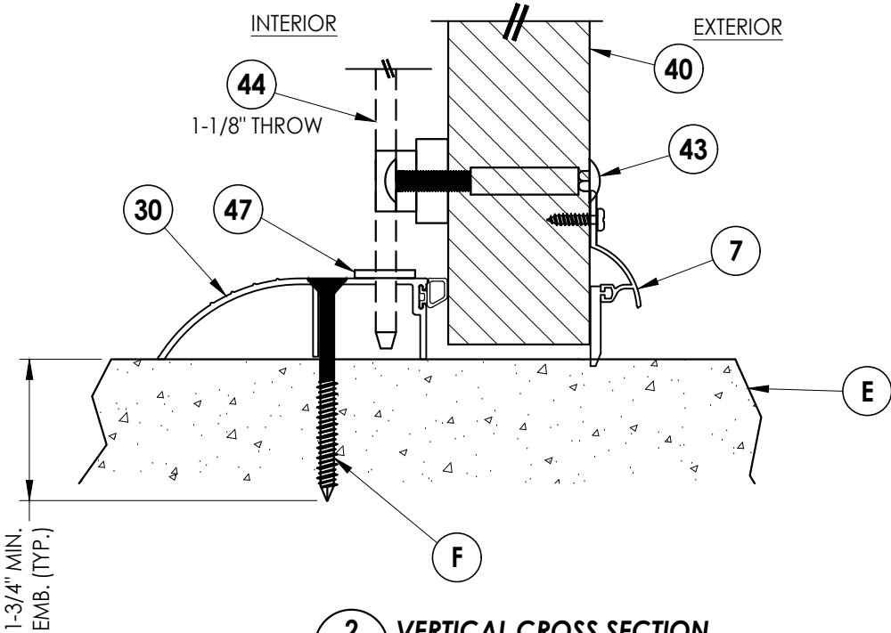
2 VERTICAL CROSS SECTION 4 Outswing Sill
