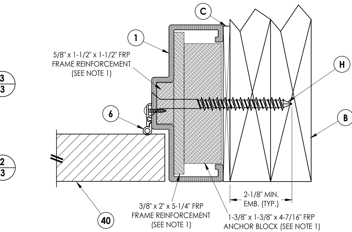
3 3 HORIZONTAL CROSS SECTION Outswing configuration
